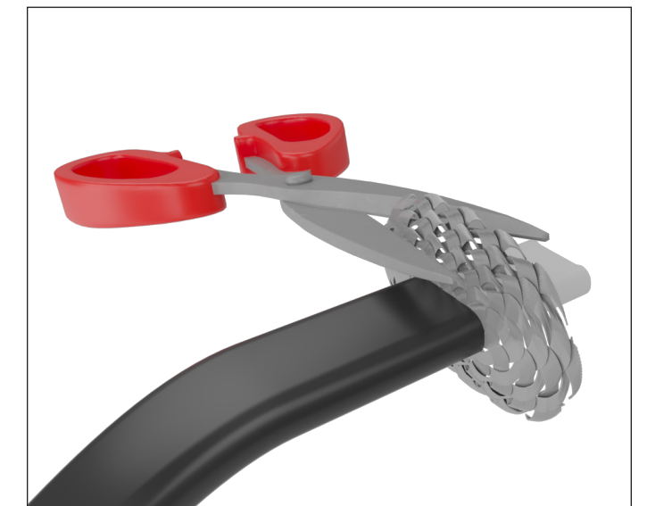
13. Trim away the exposed braid from the heat trace cable.
