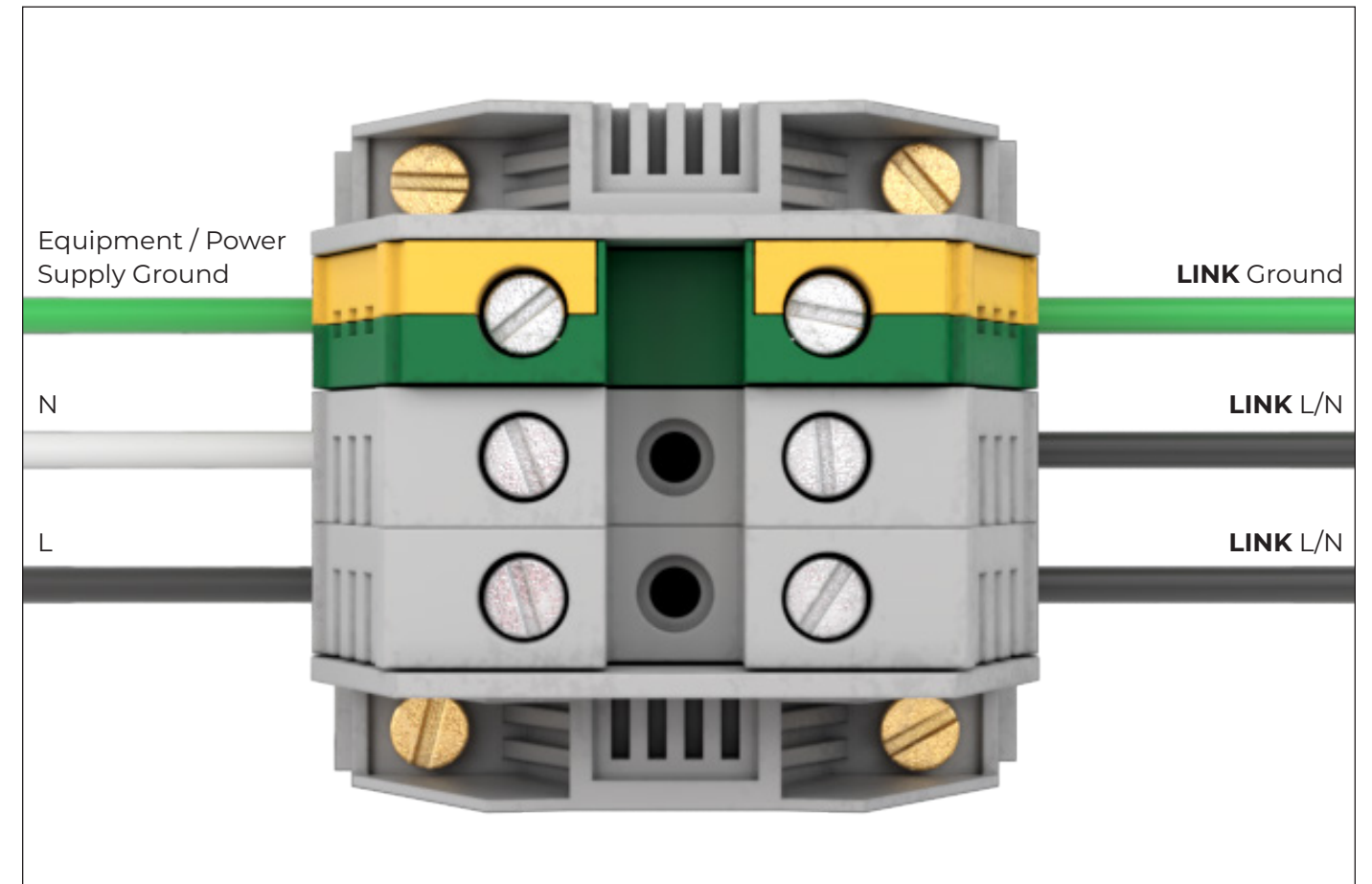
19. Complete system wiring according to customer design. Customer supplied terminal blocks, lugs, wire nuts, or other suitable and appropriately rated connection equipment to be used. Refer to typical terminal block example shown above.
