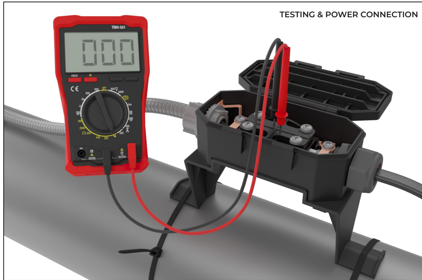
16. Test ports are included in all LINK IDC models to help the heat trace installer confirm there is continuity across the device after the connection is made. Please refer to the heat trace design guide and installation instructions for detailed information about heat trace use. Please refer to the instruction manual of the specific multimeter being used as exact details will vary by model. The basic process for continuity testing is as follows:
