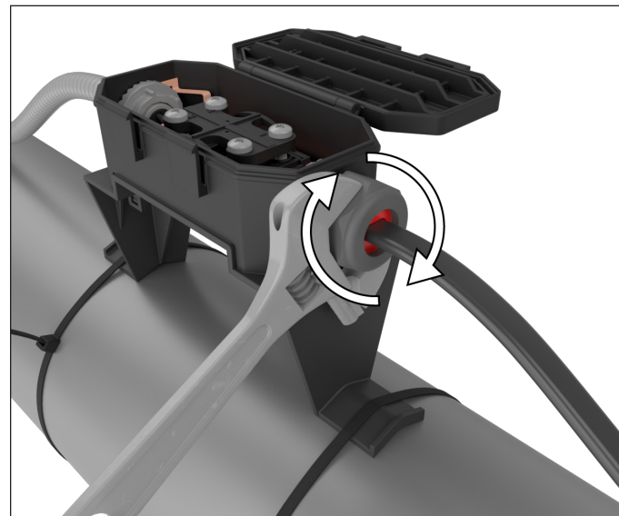
8. Torque gland nut (8 Nm for "LINK-B" version, 5 Nm for "LINK-D" version) to seal around cable.
