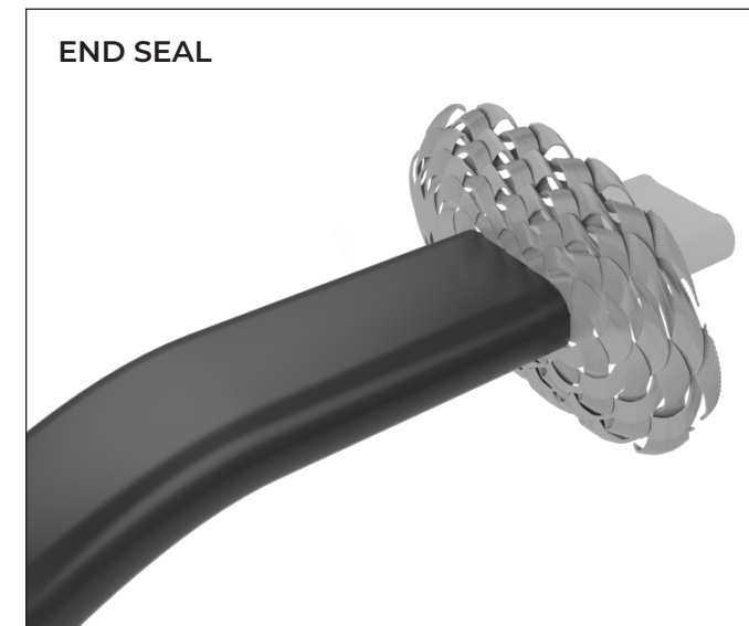
12. For installing an end seal, repeat steps 3-5 on the opposite end of the heat trace cable from the enclosure, and then pull the braid away from the cable.
