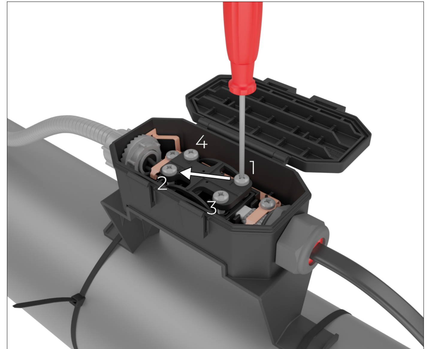
11. Starting with the screw labeled "1", and using an "X" pattern, tighten each screw approximately halfway down. Then repeat the "X" pattern until the IDC is fully seated with a torque of 2 Nm on each screw.
