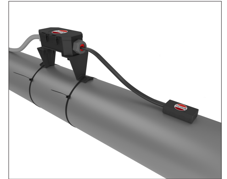
18. The heat trace circuit is now ready for taping to the piping, final electrical connections, and insulation.
