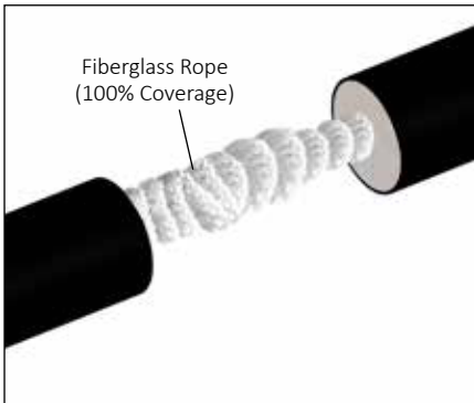
4. Wrap high temperature tubing with 1/2" fiberglass rope. Ensure 100% coverage.
