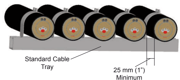
Illustration C: Typical Installation
